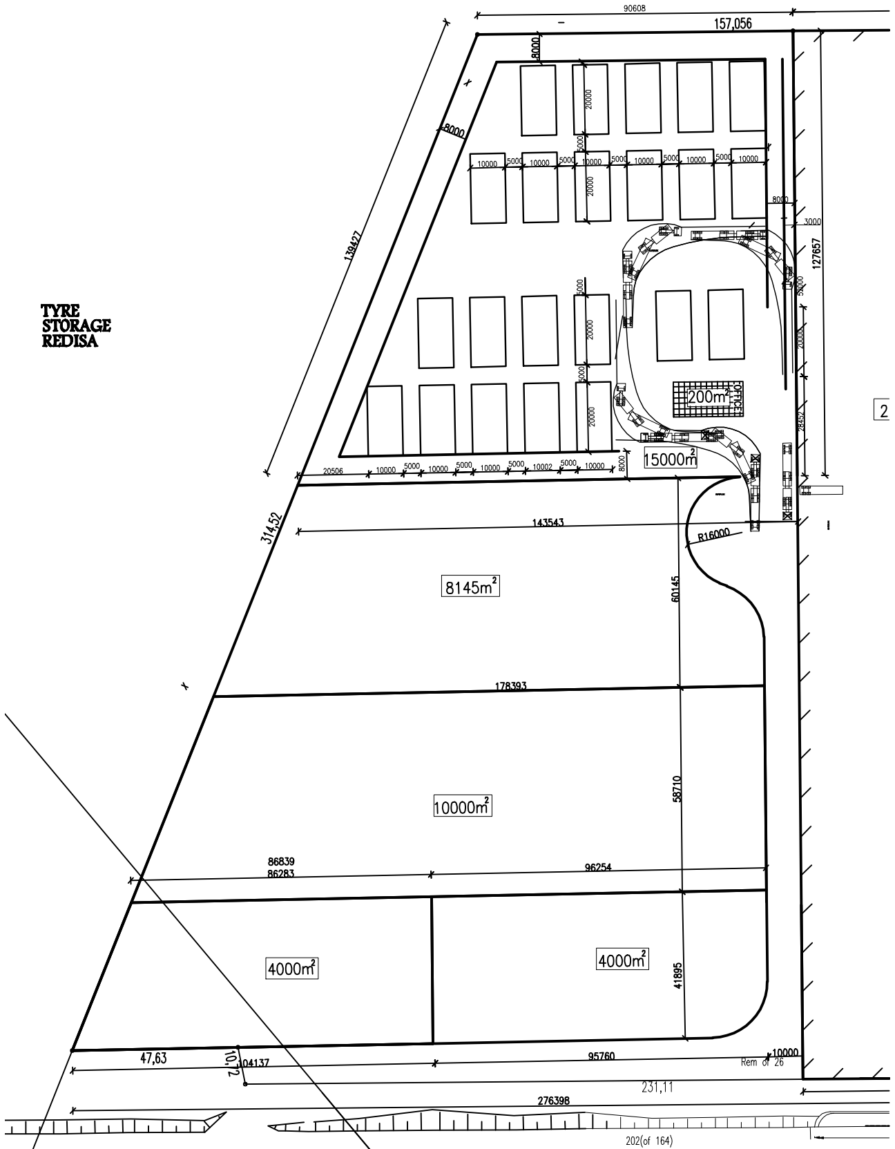
scheme 1 AIRFIELD INDUSTRIAL YARDS 1:1500
